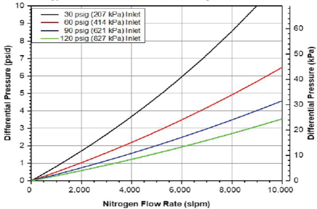
Mott BGF-310H Flow Rate vs. Differential Pressure Typical Flow Curves as a Function of System Pressures
